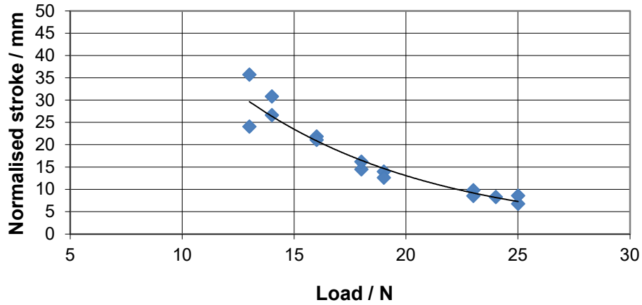
Graph of Load vs. Stroke Length
